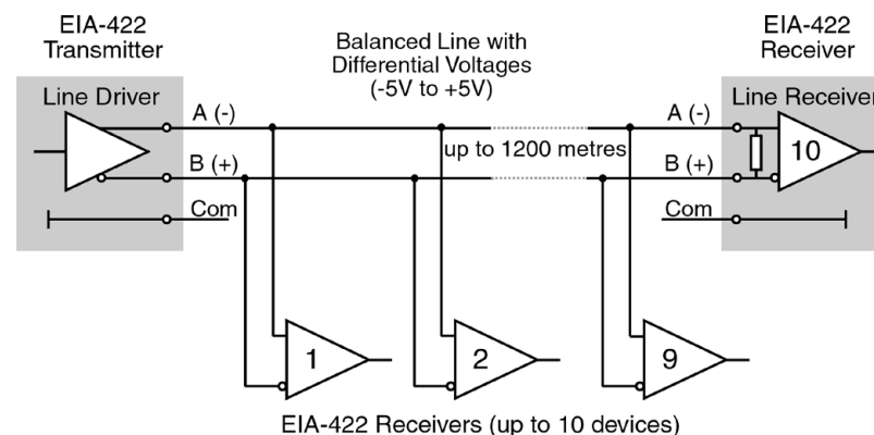
Figure 1.3 RS-422 Connection
