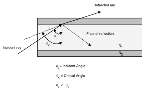
Figure 3.4 Fresnel Reflection
