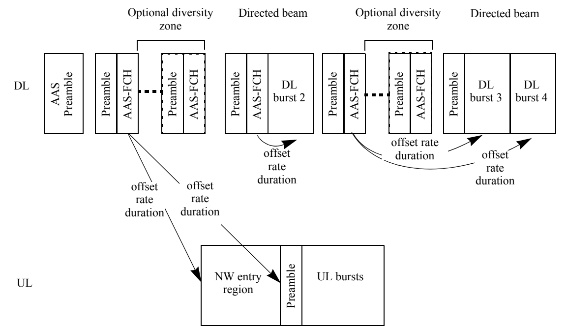
Figure 209—Structure of AAS Zone
