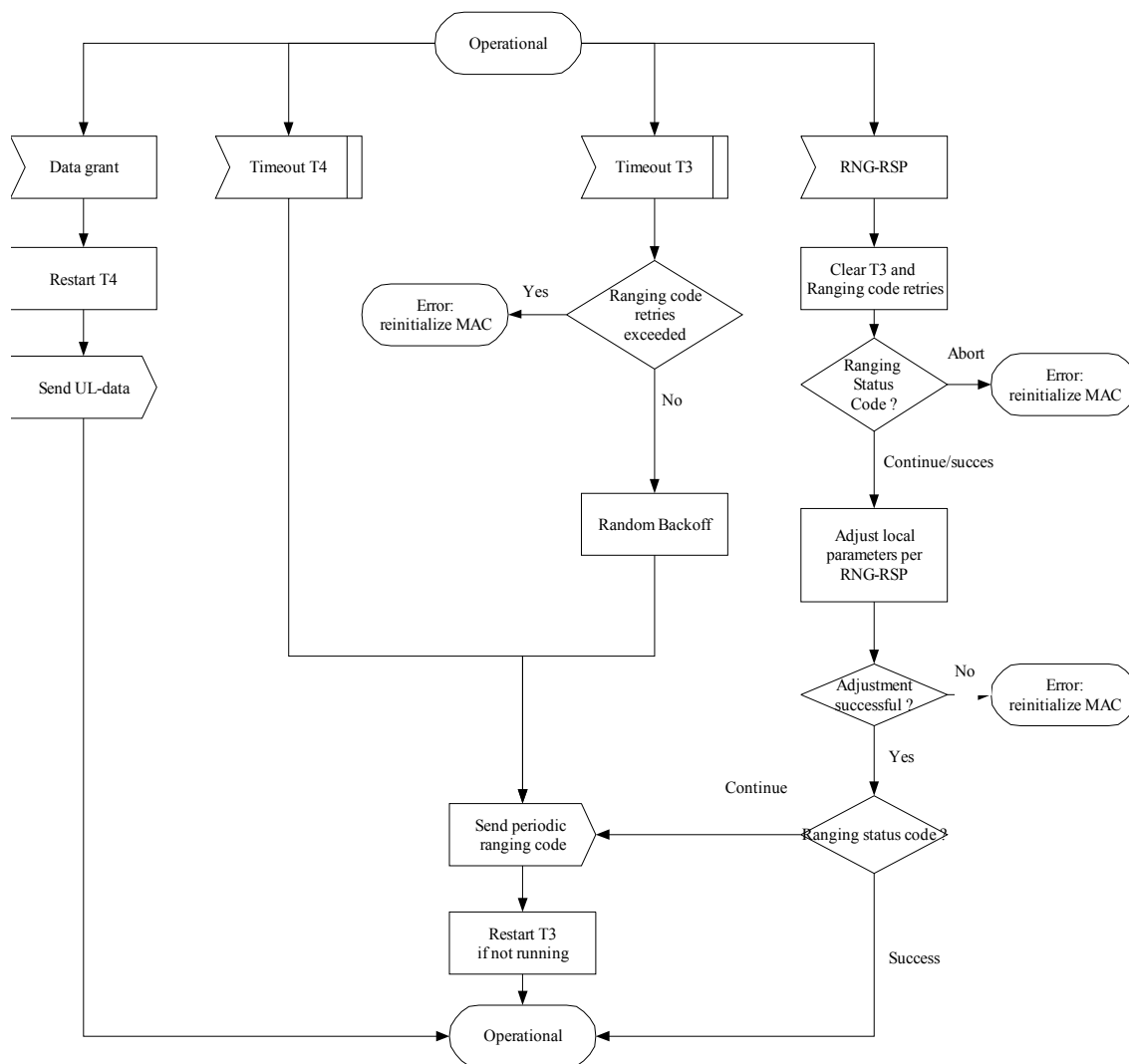
Figure 90—Periodic CDMA ranging—SS
