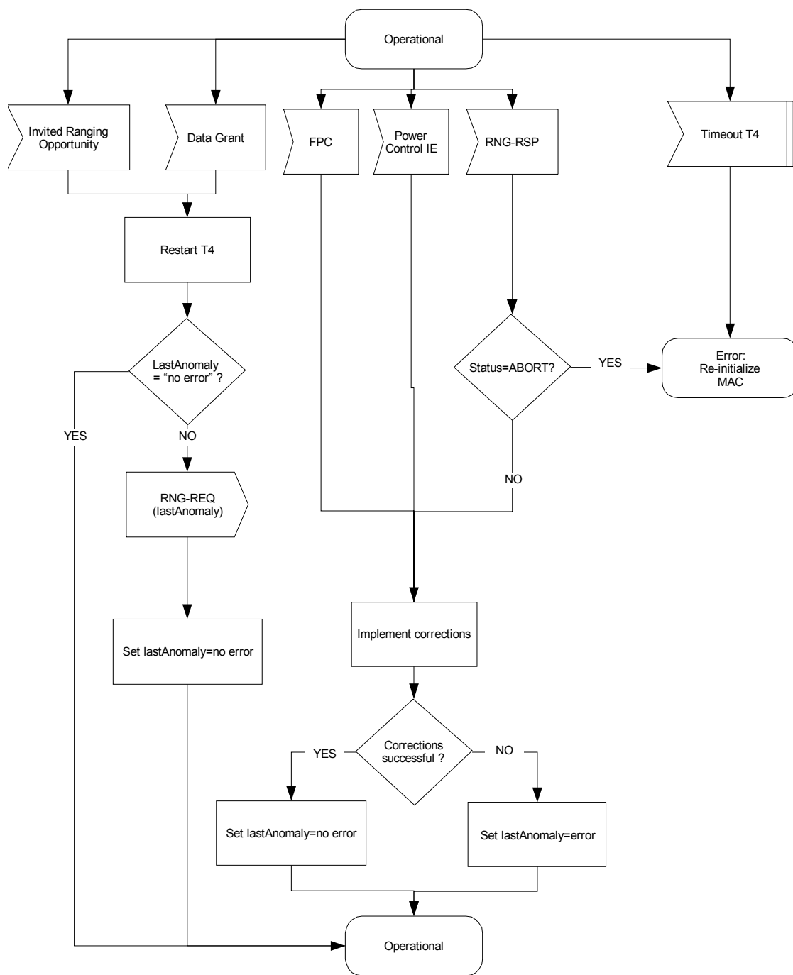
Figure 84—Periodic Ranging—SS
