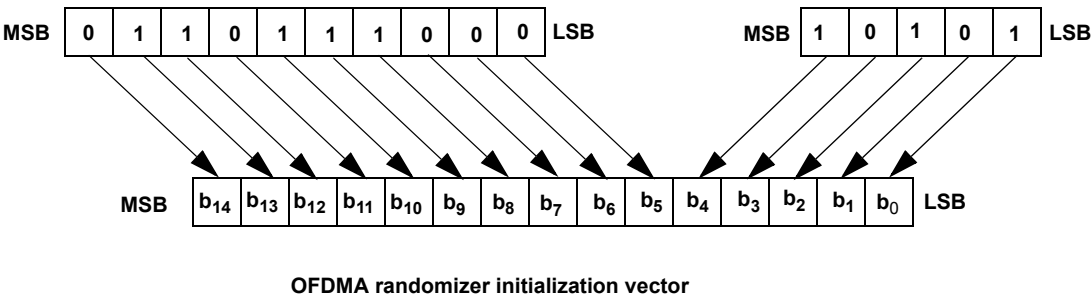
Figure 254a—Creation of the OFDMA randomizer initialization vector for HARQ
