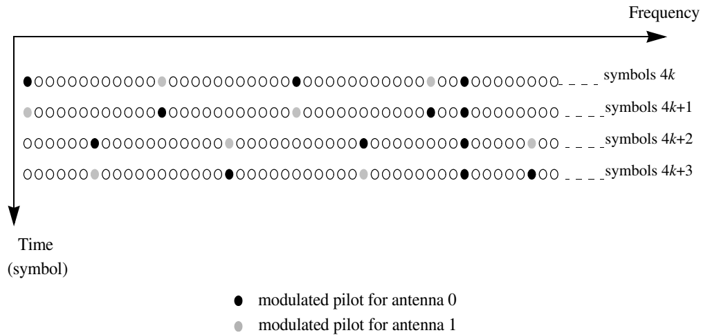
Figure 247—STC usage with FUSC
