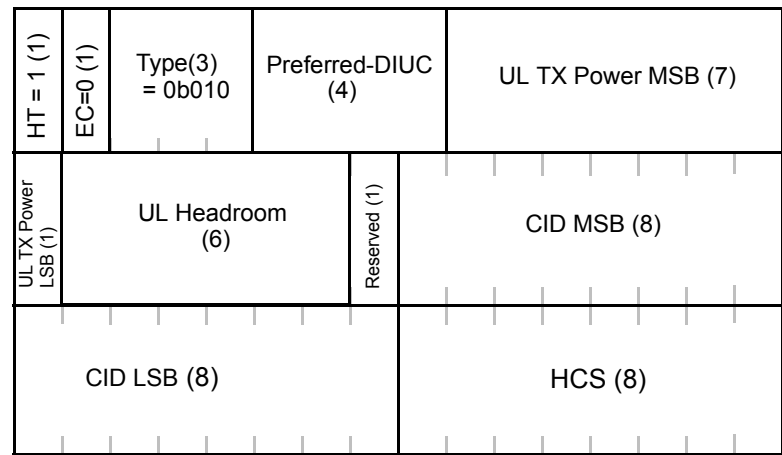
Figure 20d—PHY channel report header
