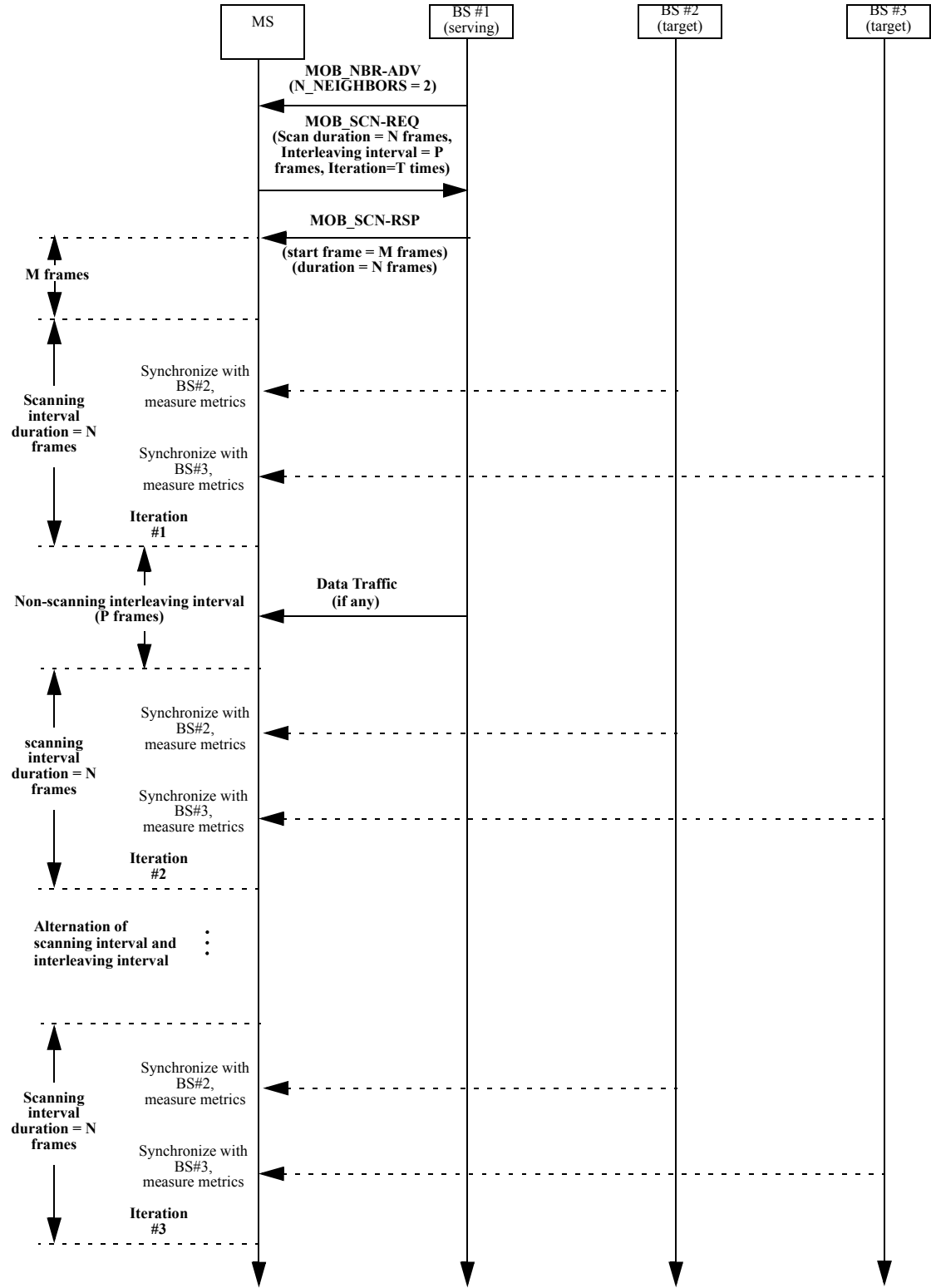
Figure D.1—Example Neighbor BS advertisement and scanning (without association) by MS request
