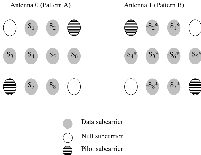
Figure 249—Mapping of data subcarriers in STTD mode
