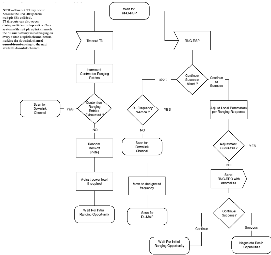
Figure 61 – Initial Ranging – SS (part 2)
