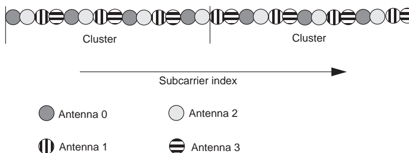
Figure 251o—Midamble PUSC structure (frequency domain)
