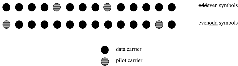
Figure 234—Cluster structure
