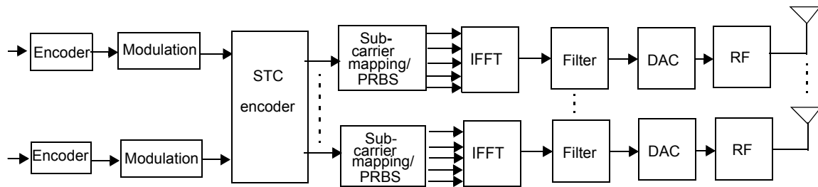
Figure 251c—Example of matrix B with horizontal encoding for 3 or 4 Tx BS for optional zones in DL
