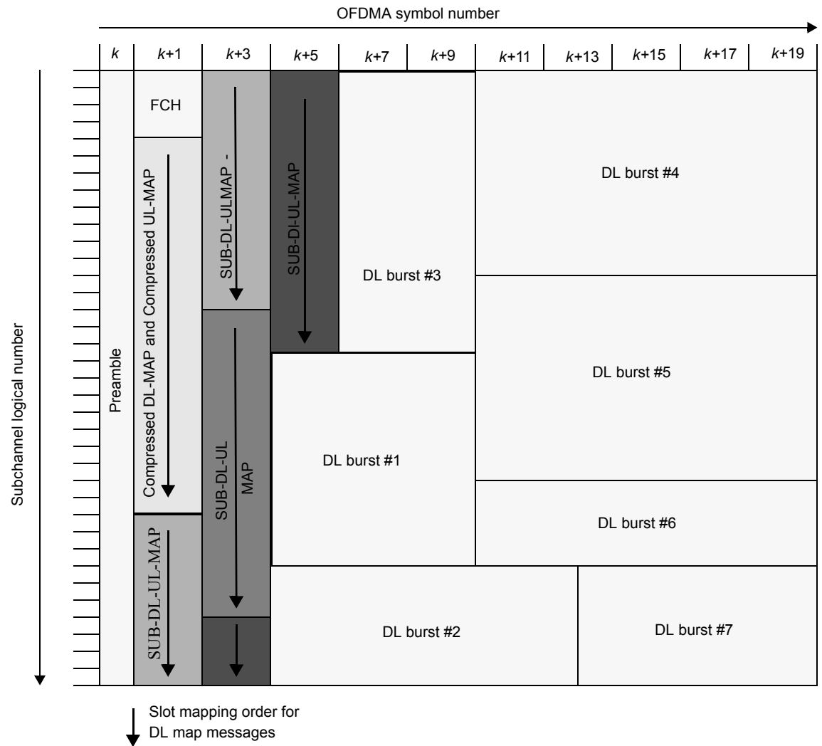
Figure 23b—Sub-MAP Burst
